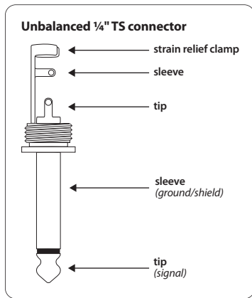
Fig. 4.3: 1/4" TS connector
