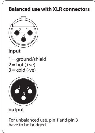
Fig. 4.2: XLR connections
